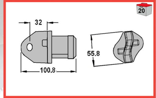
EMF635 SB35 Weld On Drive Lug
