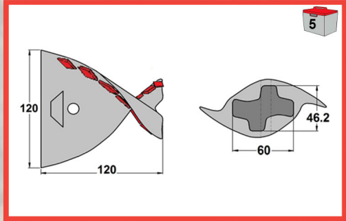
EMF611 SB45 TC, Fish Tail Pilot, Carbide Tipped
