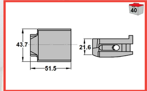
EMF660 - 35 SERIES T36, Tooth Holder
