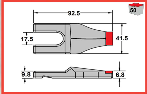
EMF508 - 35 SERIES Chisel Tooth, Carbide Tipped
