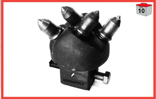
EMRP4 4 Tooth Pilot, 4" Square Shank. Takes #EMB47K19-L teeth.
