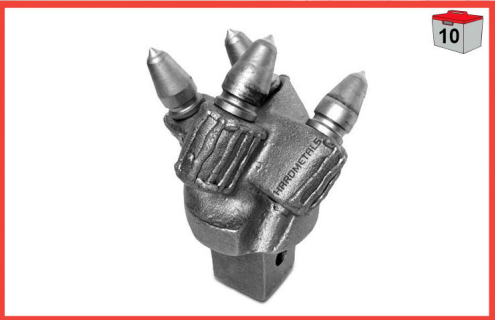
EMRP9 4 Tooth Pilot, 3-1/2" Pin. Takes #EMC31HD teeth.
