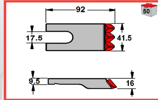
EMF535 - 35 SERIES Heavy Duty, Triple Teeth, Carbide Tipped
