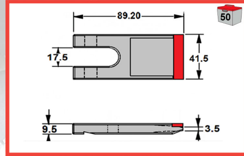
EMF527 - 35 SERIES Flat Tooth, Carbide Tipped
