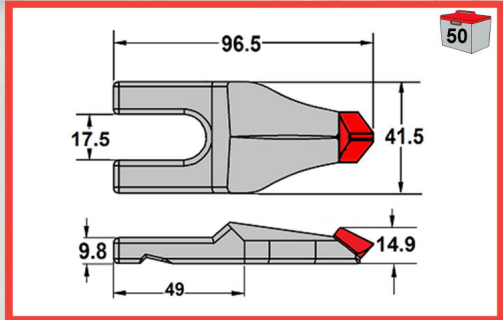
EMF509 - 35 SERIES Chisel Tooth, Carbide Tipped, FW Insert
