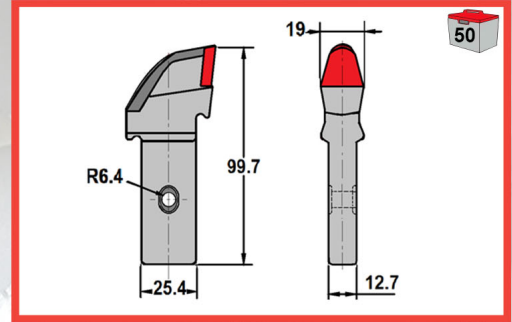
EM411-F Flat Cutter Pick, 19mm Insert
