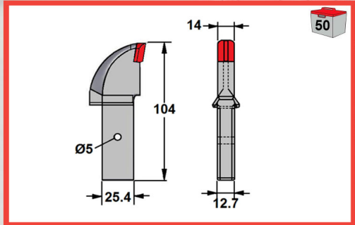
EM411-P Flat Cutter Pick, 14mm Insert (FW8B)
