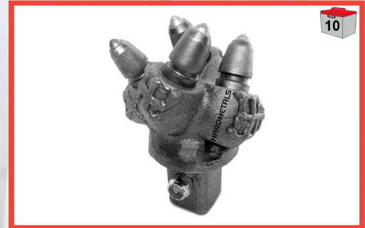
EMMM2 4 Tooth Pilot, 1-3/4" Square Shank. Takes #EMSC1-01 teeth.
