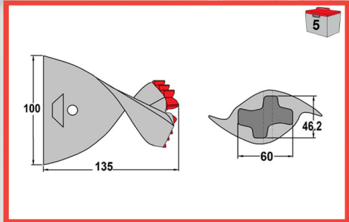
EMF612 SB35 HD TC, Fish Tail Pilot, Carbide Tipped, Heavy Duty
