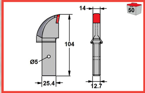
EM410A-F Flat Cutter Pick, 14mm Insert
