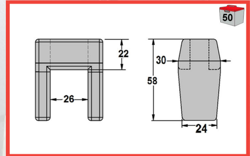
F-2S Flat Cutter Pick, Block Forged
